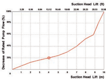
With a suction lift of 4 m, pump rate decreases by approximately 20%. Valid for pumps 3/4” and larger; data varies with pump configuration.
