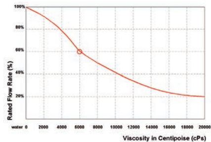
During the conveyance of a fluid with a viscosity of 6000cPs, the pump rate decreases to 60% of its rated value (100% = water). Valid for 3/4” pumps & larger.
